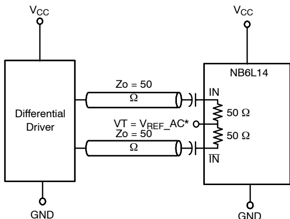
Figure 18. Capacitor-Coupled Differential Interface (VT Connected to V REFAC )
