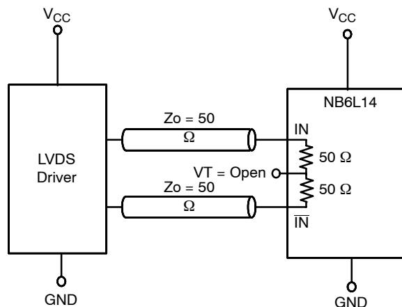
Figure 16. LVDS Interface
