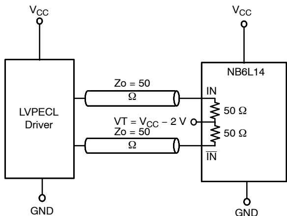
Figure 15. LVPECL Interface
